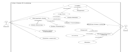
Gambar 3. Usecase Diagram
