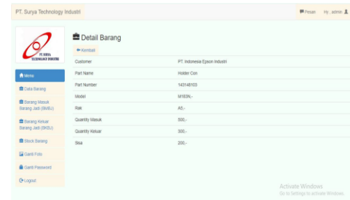
Gambar 4.5 Tampilan detail
