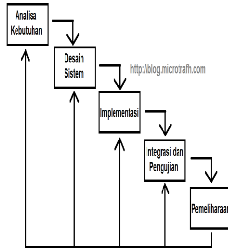
Gambar 3.1 Waterfall
