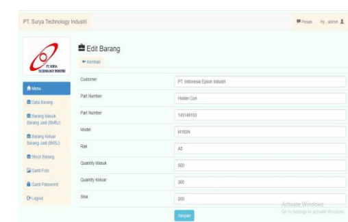
Gambar 4.7 Tampilan edit
