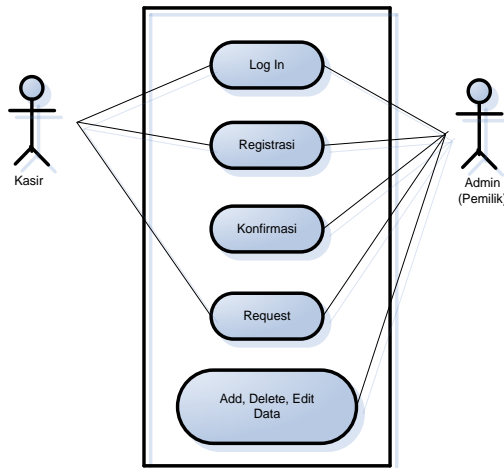
Gambar 2 Usecase Diagram
